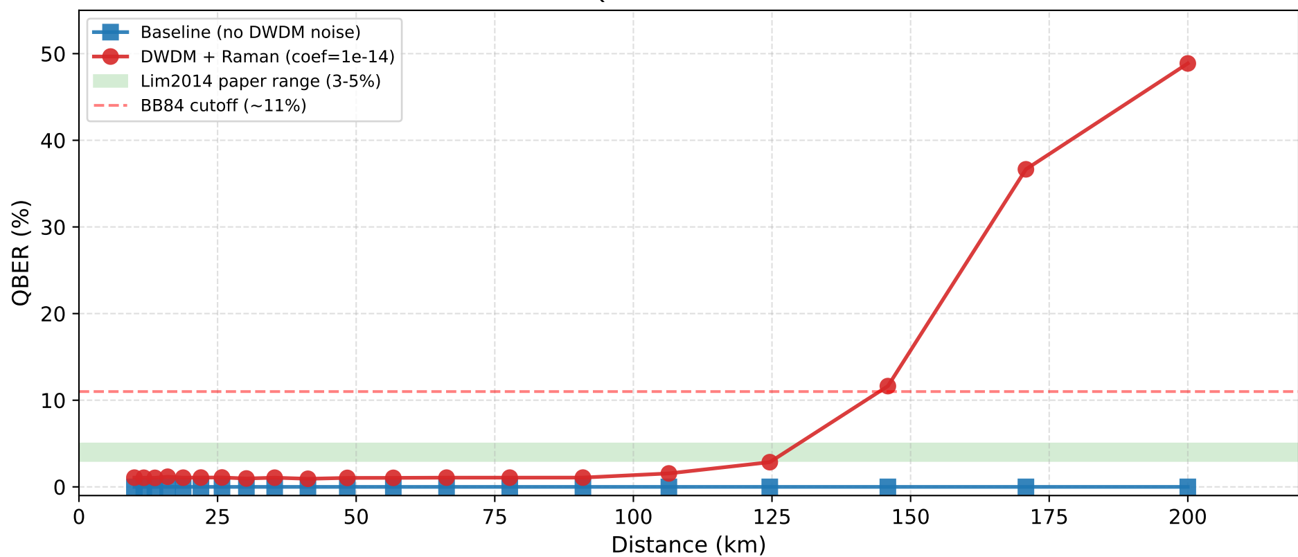
QBER vs Distance
