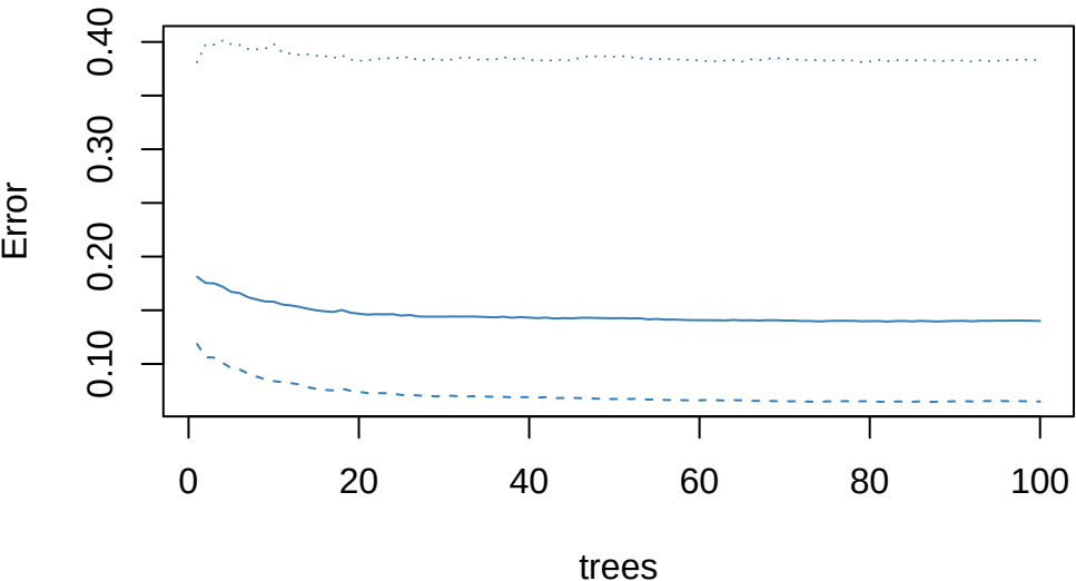
Random Forest Error Rate vs. Number of Trees
