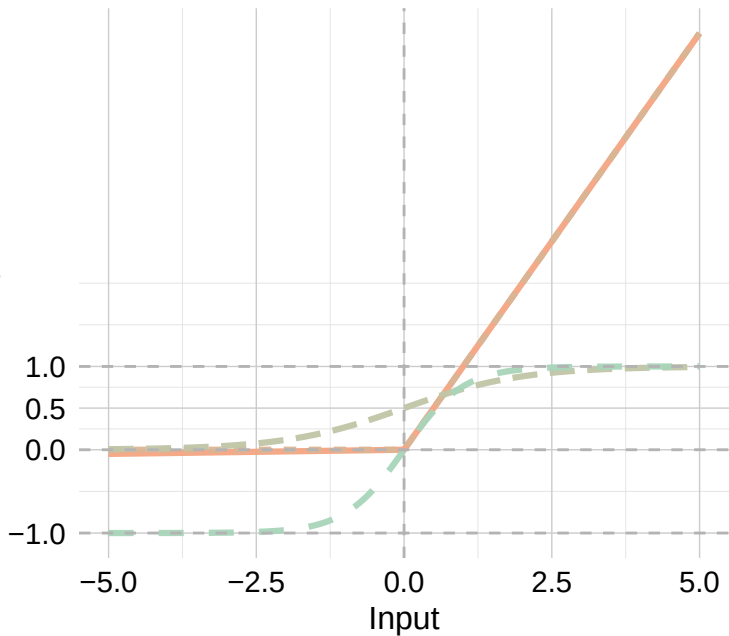
Comparison of Activation Functions
