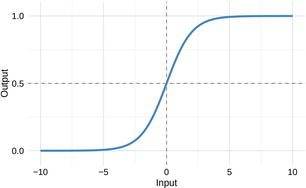
Sigmoid Activation Function
