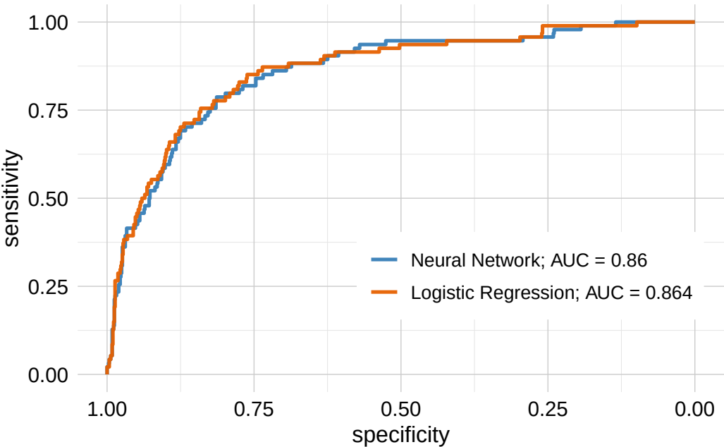
ROC Curves: Neural Network vs Logistic Regression
