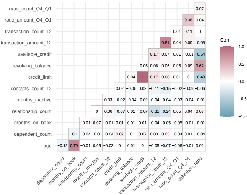
Correlation Matrix for Numerical Features
