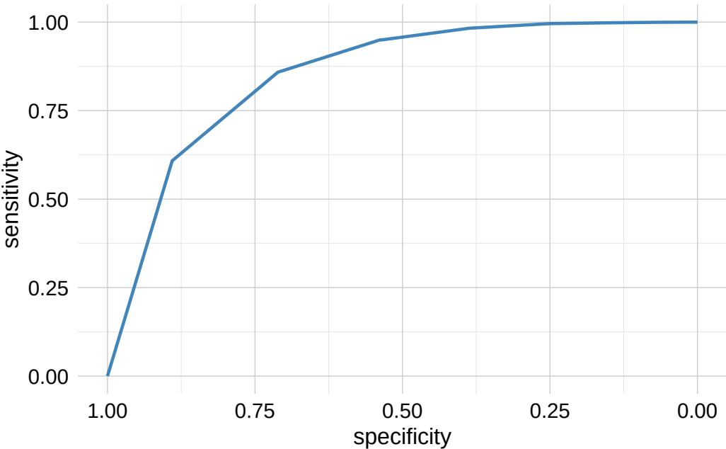
ROC Curve for the kNN Model on the churn Data
