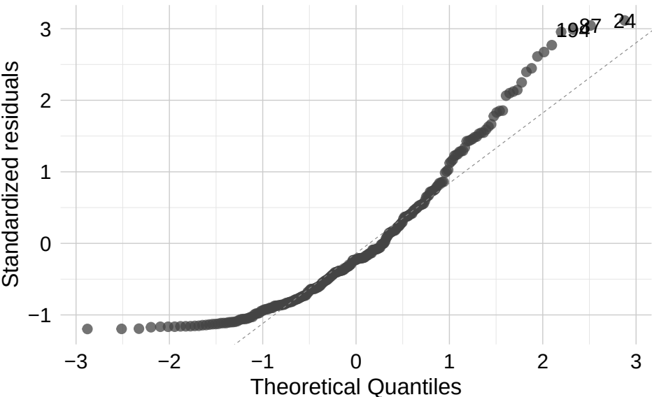
Simulated non-normal residuals
