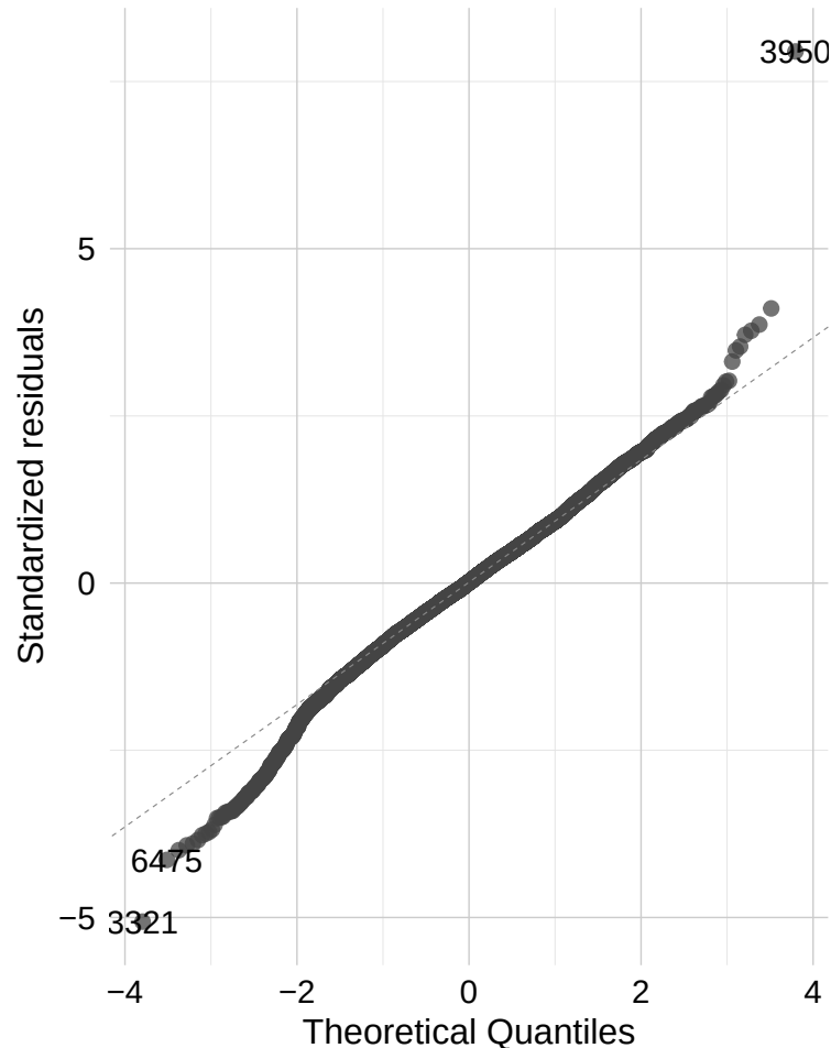
Selected regression model
