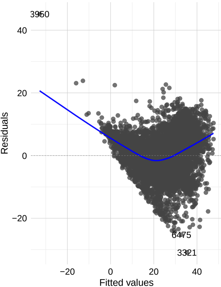
Selected regression model
