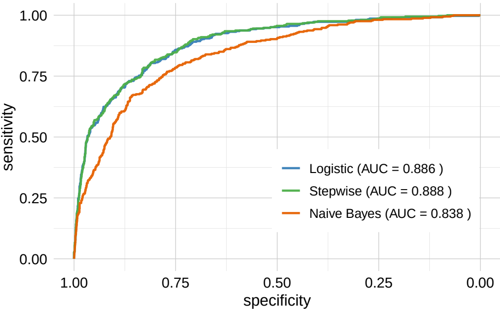
ROC Curves for Three Classification Models
