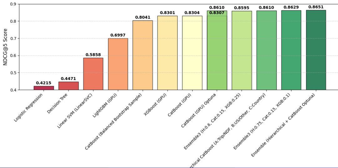
Detailed Model Comparison: NDCG@5 Score
