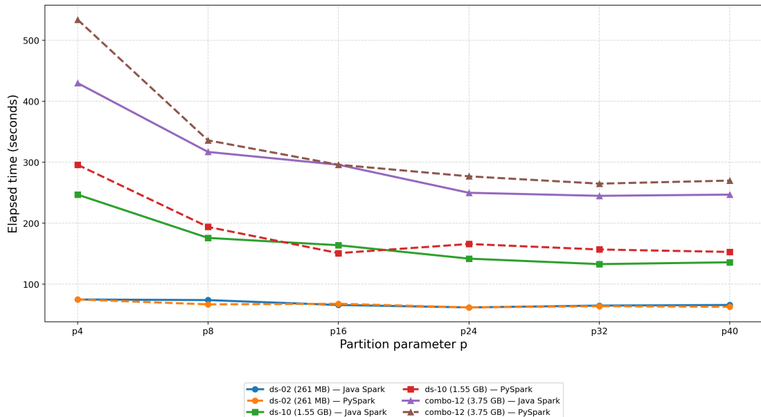
Figure 2 — Spark Partition Sweep: Elapsed Time vs p
