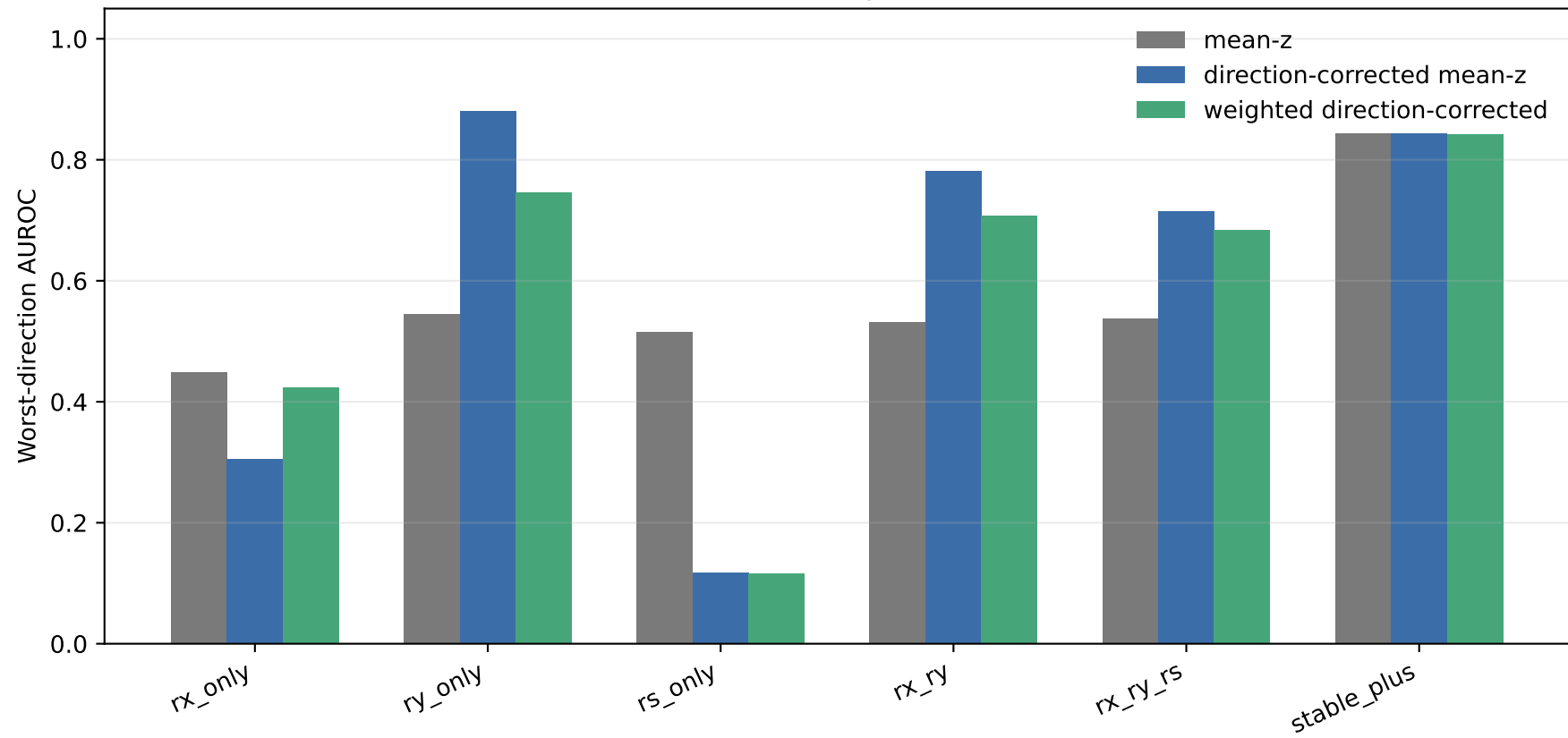
Channel/family ablation
