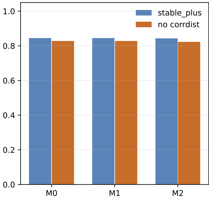
Worst AUROC
