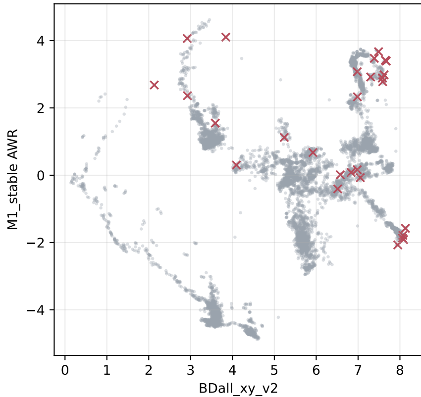
Exp1: candidate AWR-BD map
