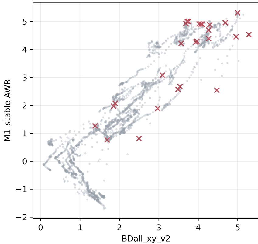
Exp2: candidate AWR-BD map
