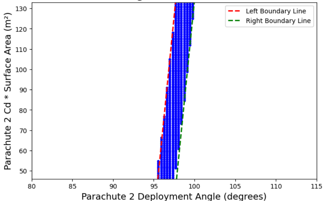
Figure 15. Graph of all combinations of C = C_d \times A and deployment angle where final rocket position is 100m from original launching position. The valid values create a parallelogram defined by
