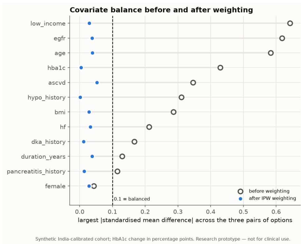
Figure 5.3: Covariate balance before and after weighting (target: standardised difference below 0.1 [31])
