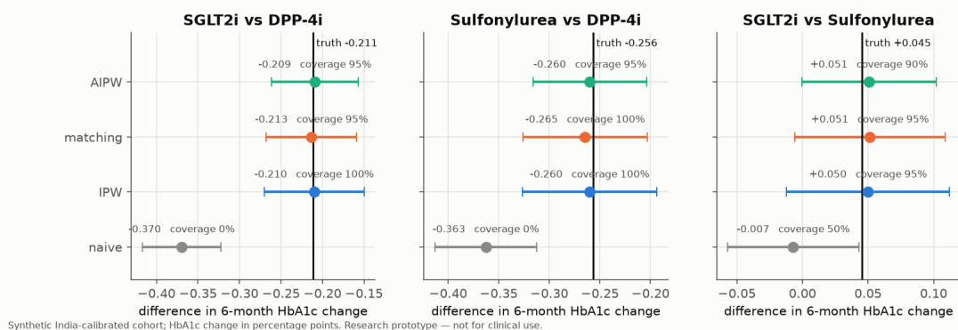
Average effect: estimate and 95% CI (averaged over repeats) vs the true value
