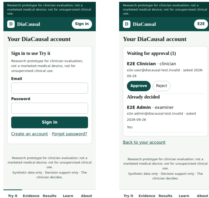
Figure 5.12: Phone website: sign-in (left) and the admin's approval screen with test accounts (right)
