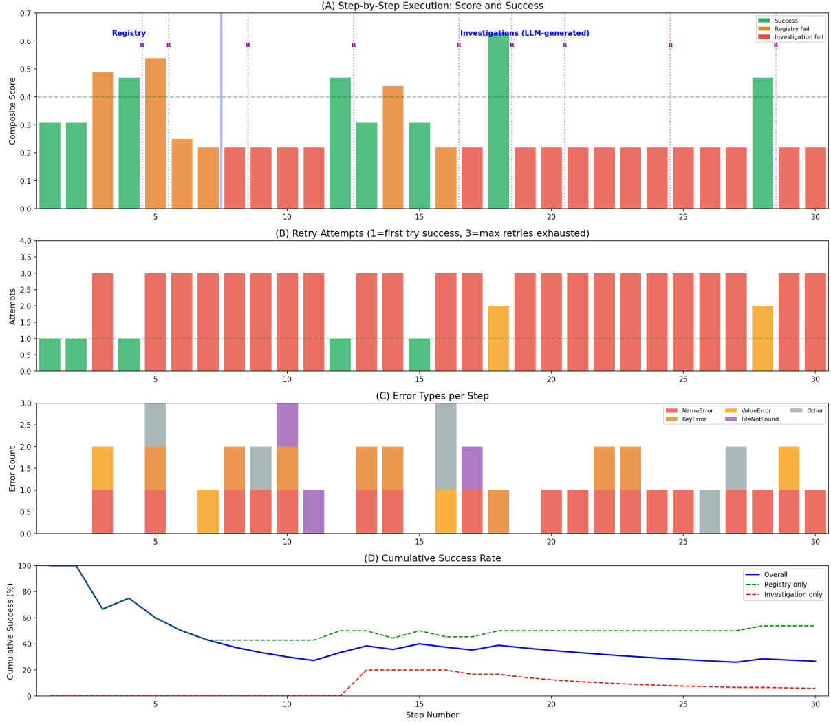
Figure 6: Execution timeline (30 steps). (A) Composite score per step; green = success, orange = registry failure, red = investigation failure; “R” = replanning event. (B) Retry attempts per step. (C) Error types per step. (D) Cumulative success rate by step type.
