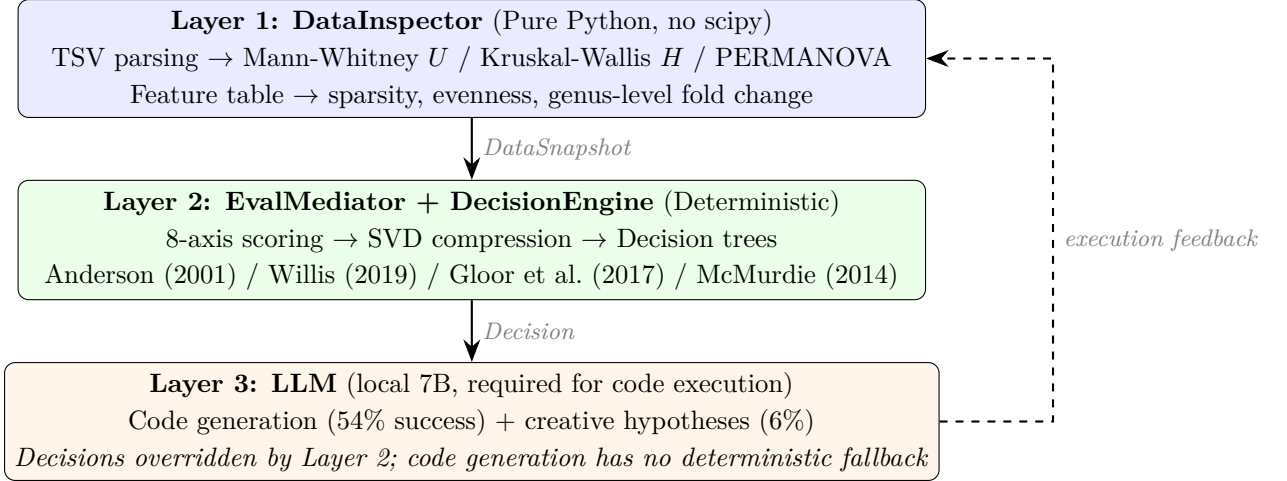
Figure 1: Three-layer architecture. Layers 1–2 are fully deterministic and LLM-independent; they handle all workflow decisions (skip, add, reorder). Layer 3 provides the LLM for code generation and is required for step execution, but its decisions are overridden by Layer 2 on conflict. The dashed arrow indicates the closed-loop feedback path.
