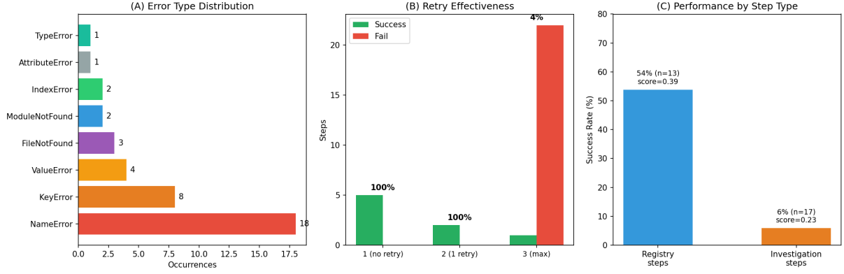
Figure 9: (A) Error distribution. (B) Retry effectiveness. (C) Step type performance.
