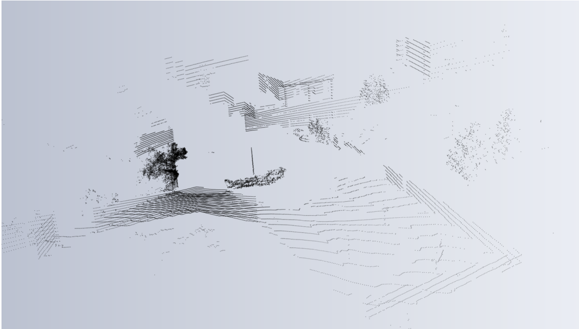
FIGURE 4.7 – Trame LIDAR
