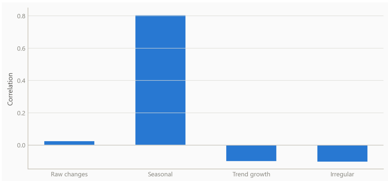
Figure 3: Correlation of the same simulated pair, measured on the raw changes and on each decomposed component (simulated data).
