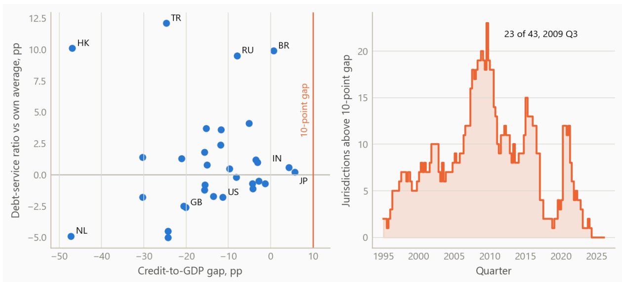
Figure 3: Early-warning screen, private non-financial sector. Left: credit-to-GDP gap against the debt-service ratio's deviation from its own average over its history (from 1999 at the earliest), 32 jurisdictions, first quarter of 2026; the vertical line marks a 10-point gap. Right: number of jurisdictions with a gap above 10 points, out of the 33 to 43 reporting each quarter, 1995 to 2026. Source: BIS credit-to-GDP gap and debt-service ratio statistics, downloaded 8 October 2026; the author's calculations.
