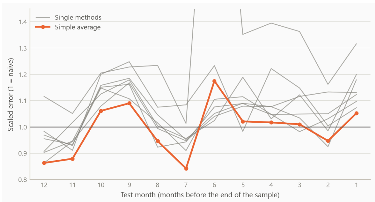
Figure 2: Mean scaled error in each of the twelve one-month-ahead tests, 181 components, against the naive benchmark at 1.0. Grey: the single methods; orange: their simple average. Tests run from twelve months before the end of the sample (left) to one month before (right). One method reaches 2.48 in the test six months back, above the top of the scale. Source: October 2025 re-run of the comparison (seven distinct methods); author's calculations.
