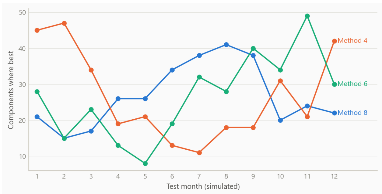
Figure 3: Number of components for which each of three methods is best, test by test (simulated data).
