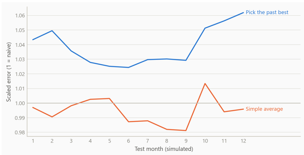
Figure 4: Out-of-sample scaled error test by test: choosing the best past method per component versus the simple average (simulated data).
