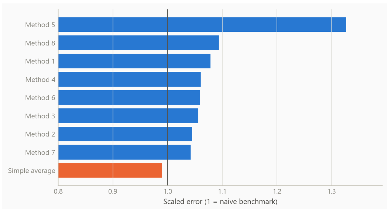
Figure 1: Mean scaled error over all twelve tests and 181 components, by method, against the naive benchmark at 1.0. Source: summary results of the comparison (September 2025); author's calculations.
