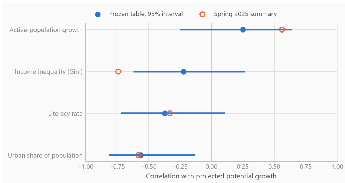
Figure 1: Correlation of each indicator with projected potential growth, 18 emerging economies, 2024-2044. Filled dots: frozen final table, with 95% intervals. Hollow dots: values in the spring 2025 summary. Source: the project's final 18-economy table (published population projections, long-run growth scenarios and development indicators); the author's calculations.
