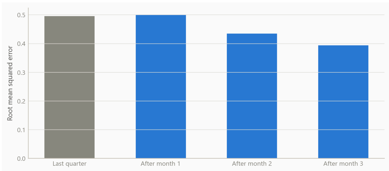
Figure 2: Average error of the current-quarter nowcast by how many months of data are in, against a naive benchmark (simulated data).
