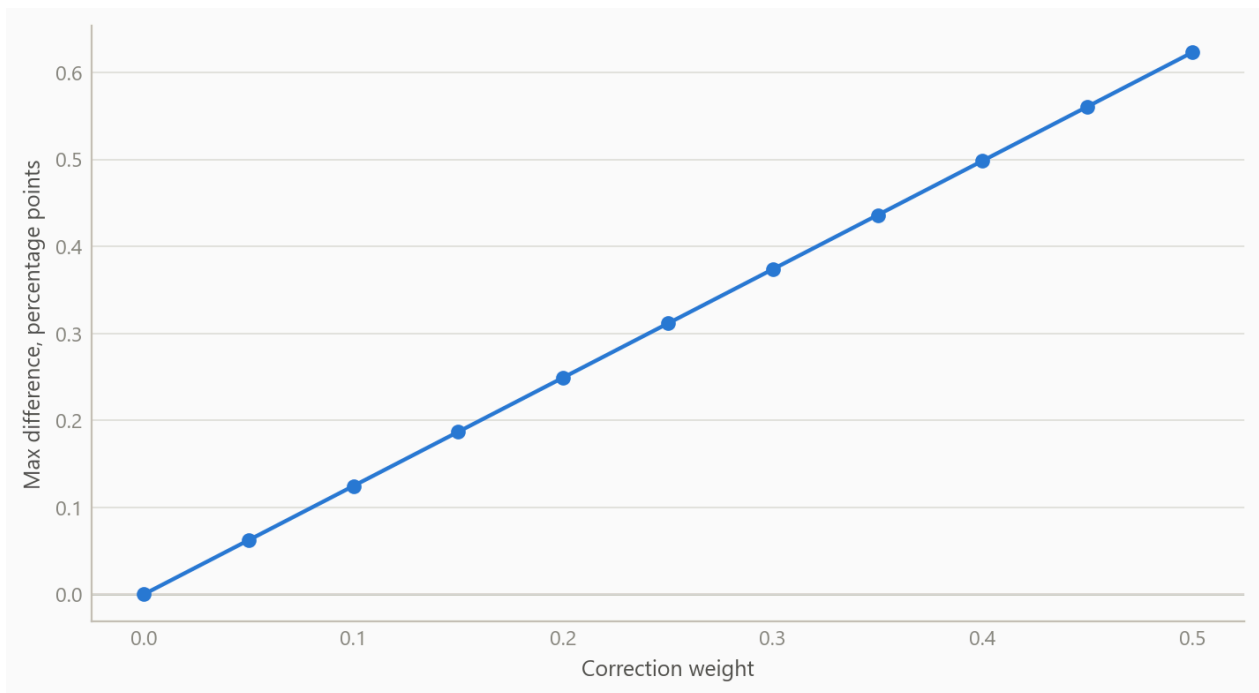
Figure 3: Largest forecast difference between a run with the optional correction and the baseline run, by correction weight (simulated data).
