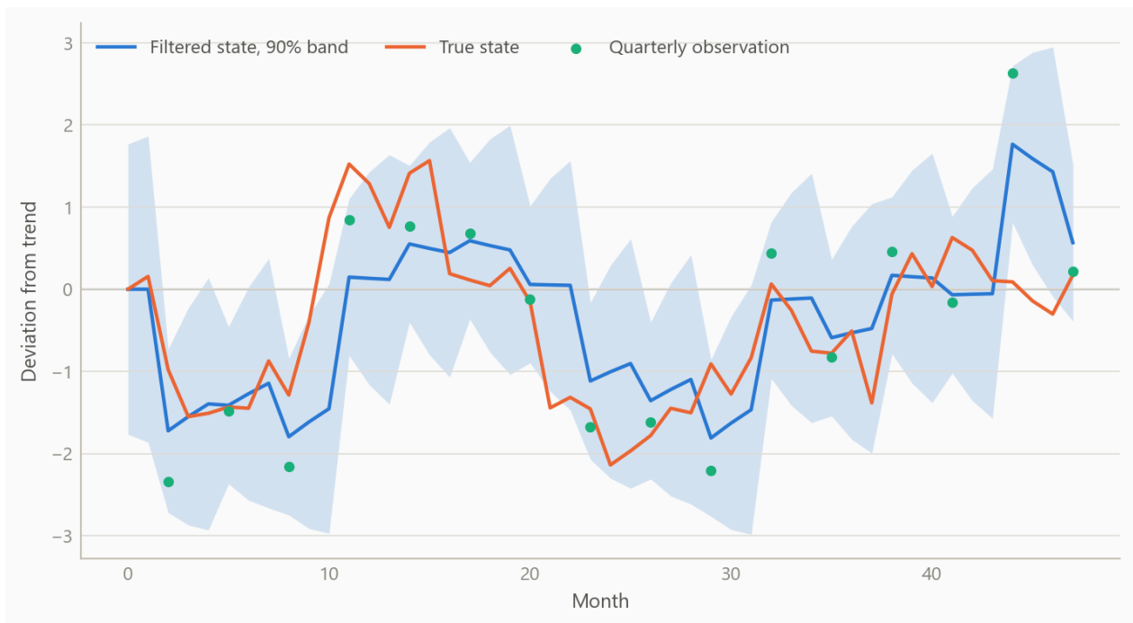
Figure 1: A latent monthly state recovered by a filter when only every third month is observed, against the known truth (simulated data).
