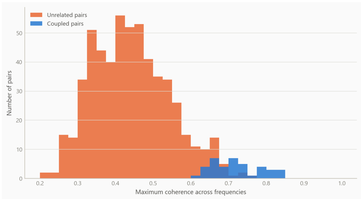
Figure 3: Maximum coherence across 600 simulated pairs, 5 per cent of which share a common cycle (simulated data).
