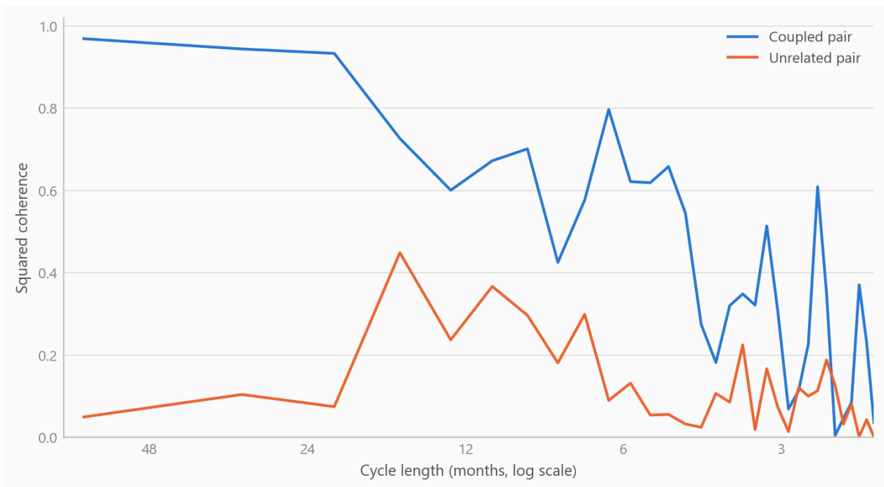
Figure 2: Coherence by cycle length for a coupled pair and an unrelated pair of monthly residual series, 300 months (simulated data).
