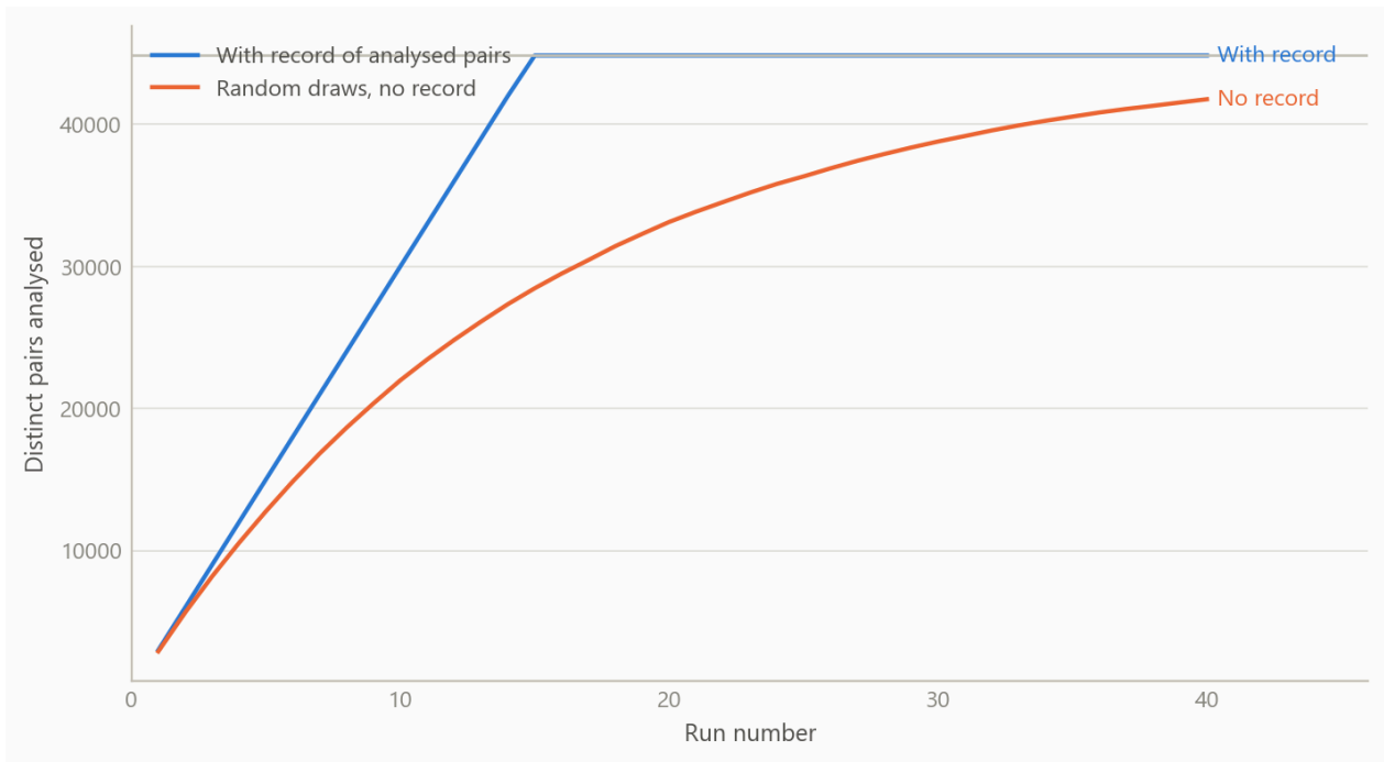
Figure 1: Cumulative number of distinct pairs analysed, with and without a persistent record, in a scaled-down universe of 300 series (simulated data).
