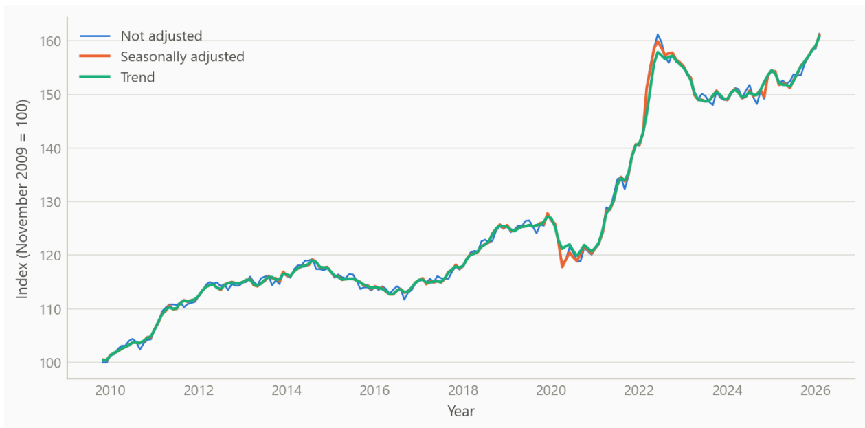
Figure 1: US producer prices for transportation and warehousing services: not seasonally adjusted, seasonally adjusted, and the trend from the airline-model decomposition, November 2009 to March 2026.
