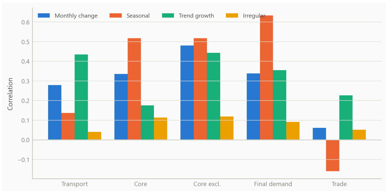
Figure 3: Correlation of each producer-consumer pair, measured on monthly log changes and on each decomposed component. Source: BLS via FRED; the author's decomposition and calculations.
