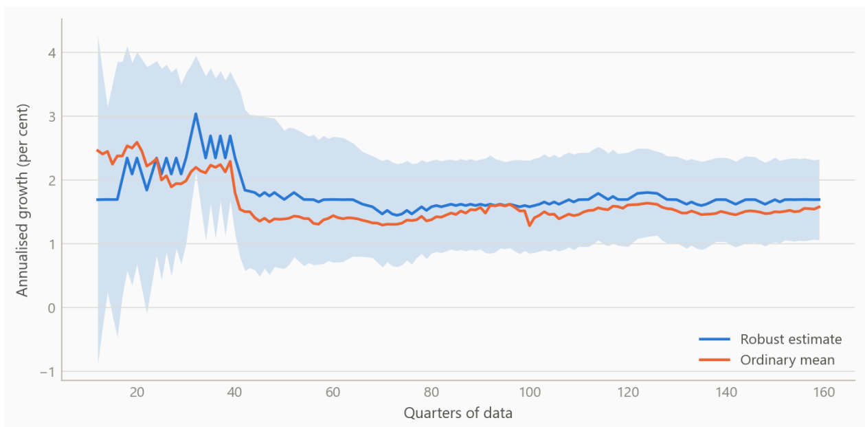
Figure 4: Long-run growth of a simulated quarterly series with crisis outliers: the robust estimate against the ordinary mean, with a 95% band that tightens as data arrive (simulated data).
