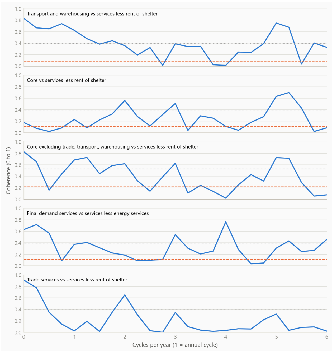
Figure 2: Coherence of monthly log changes for the five producer-consumer pairs, by cycle length. Dashed: the squared ordinary correlation. Dotted: the 95% threshold for coherence under no relationship. Source: BLS via FRED; the author's calculations.
