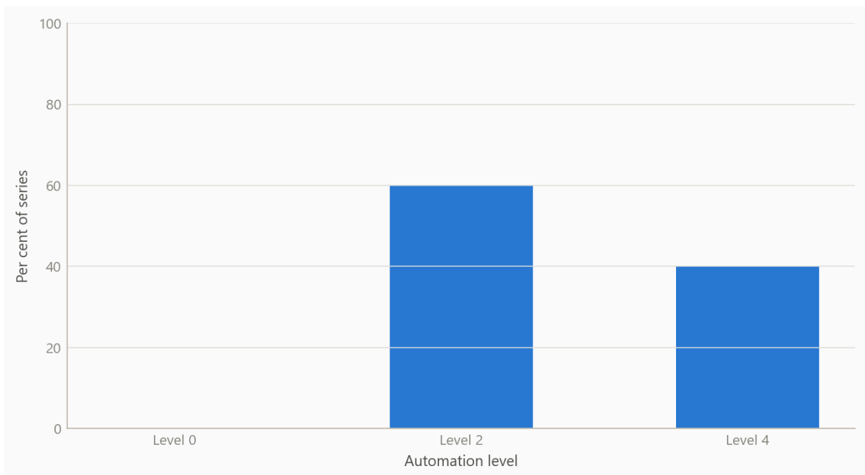
Figure 3: Share of series with a non-airline model, by automation level (simulated data, ten series per level). Levels that still run model identification can return richer models.
