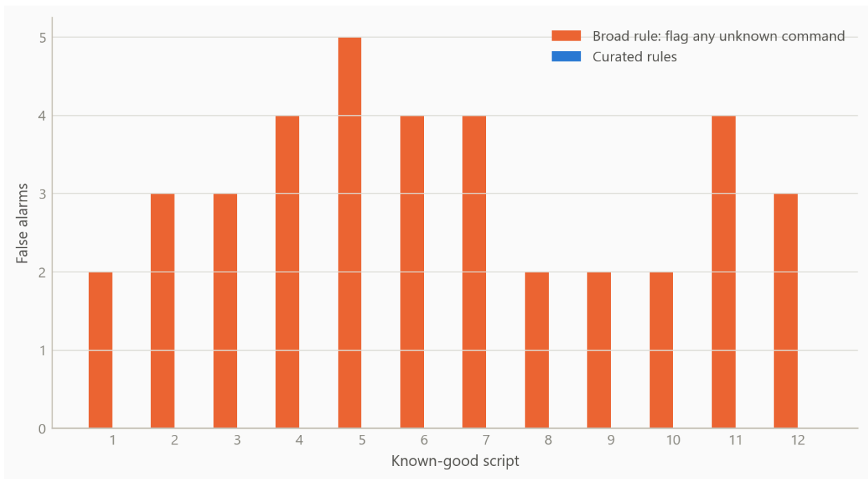
Figure 2: False alarms per known-good script under two checking designs (simulated data). The broad rule fires on correct code; the curated rules stay silent.
