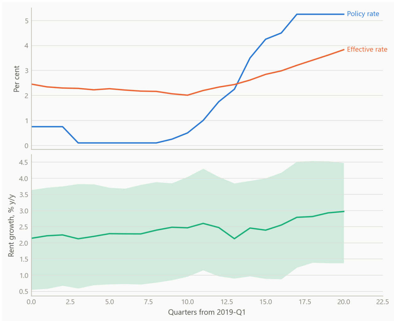
Figure 1: The two series the design compares, and the spread it exploits (simulated data). Top: policy rate and effective mortgage-stock rate. Bottom: year-on-year rent growth across 290 authorities, median with 10th to 90th percentile band.
