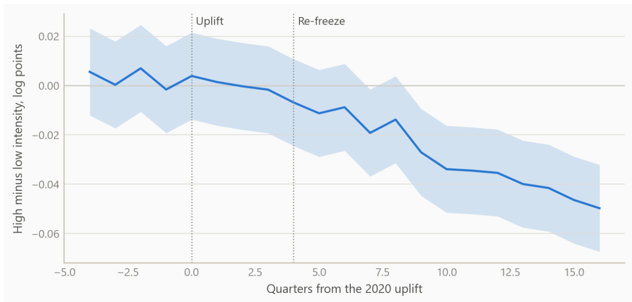
Figure 3: The shape of an event-study on benefit intensity (simulated data). Differential rent growth of high- relative to low-intensity authorities, with the uplift and the re-freeze marked. Simulated to illustrate the design, not the estimates.
