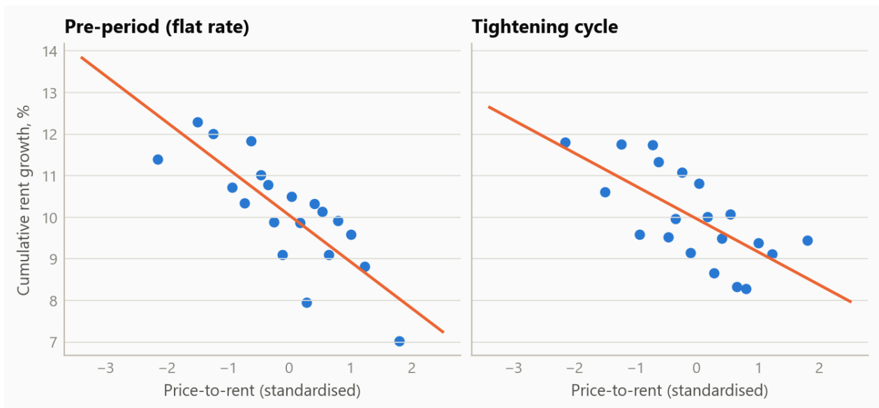
Figure 2: Why a panel and not a cross-section (simulated data). In both a flat-rate pre-period and the tightening cycle, areas with higher price-to-rent grew rents more slowly. The gradient predates the rate rises, so it cannot be a rate effect.
