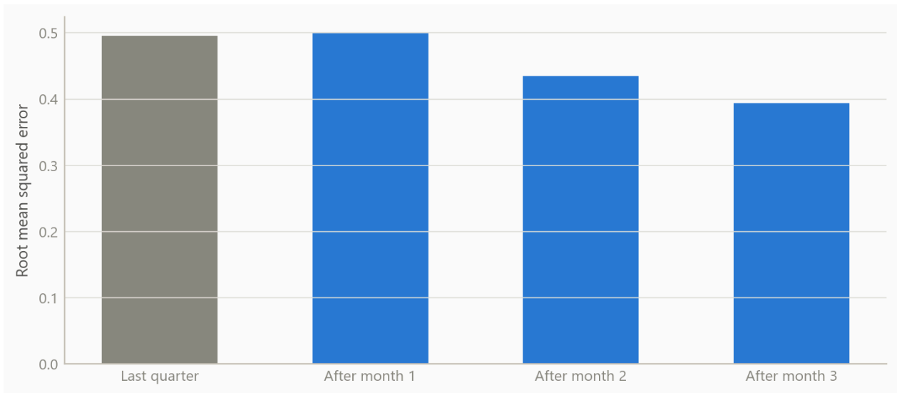
Figure 2: Average error of the current-quarter nowcast by how many months of data are in, against a naive benchmark (simulated data).
