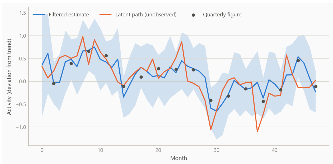
Figure 1: A monthly latent activity path, noisy quarterly averages observed at quarter-end, and the filtered estimate with its band (simulated data).
