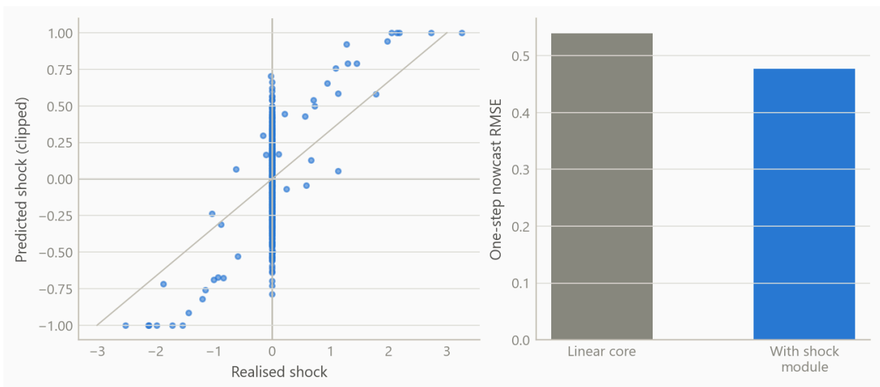
Figure 3: Left: shocks predicted by the learned module against realised shocks, clipped at a bound. Right: nowcast error with and without the module (simulated data).
