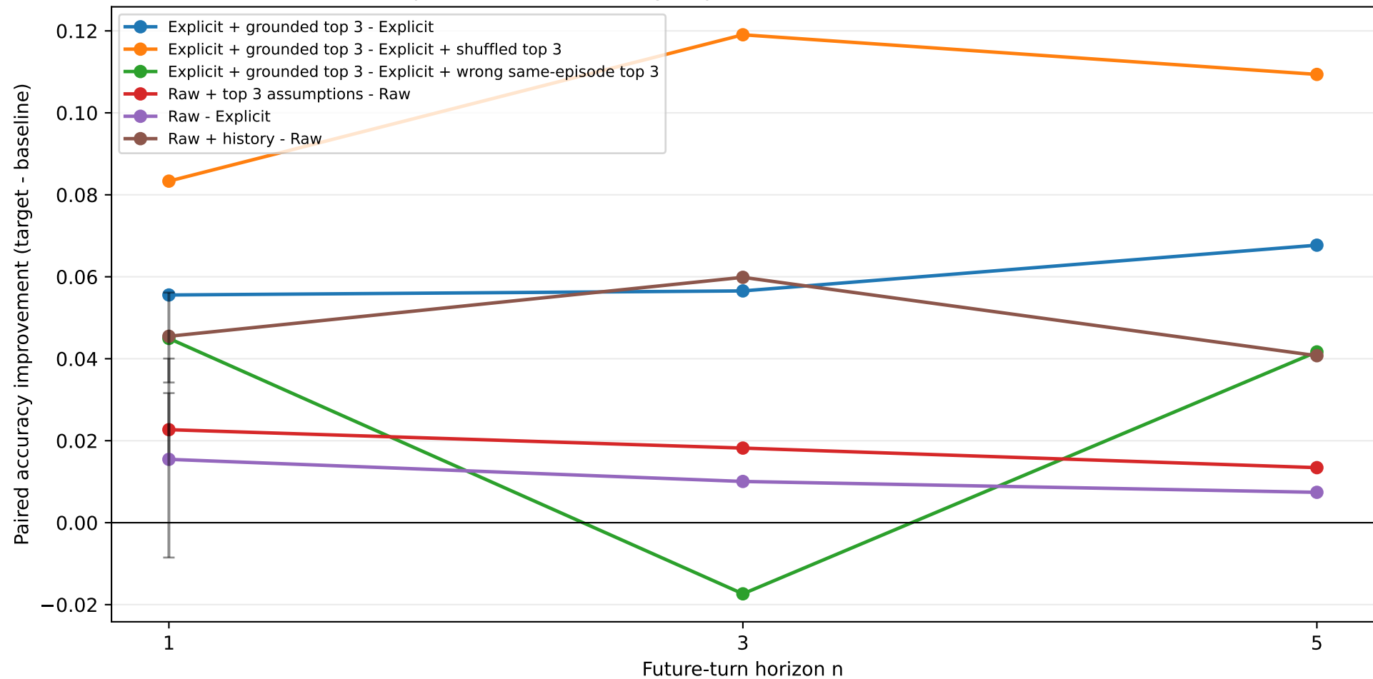
Representation accuracy improvements across future horizons
