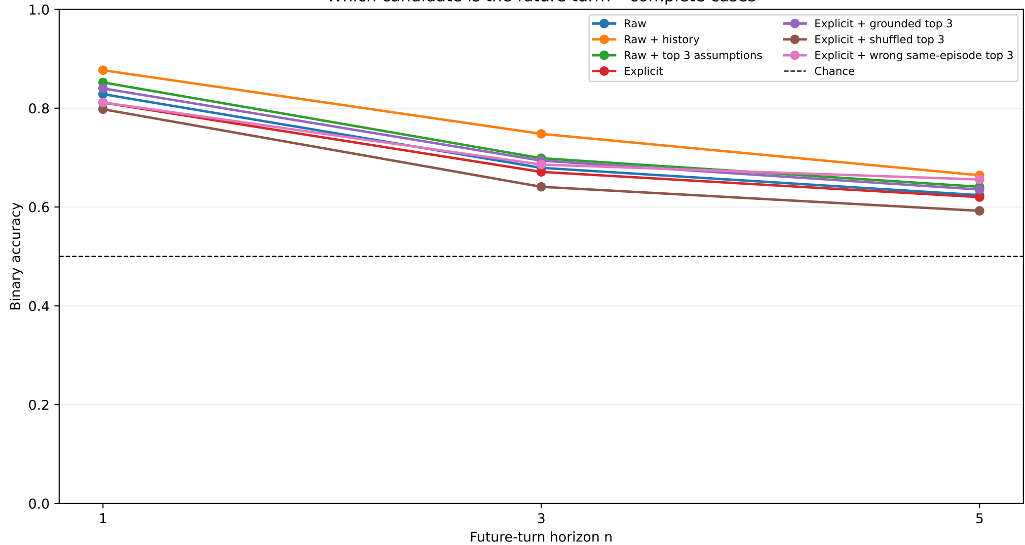
Which candidate is the future turn? - complete cases
