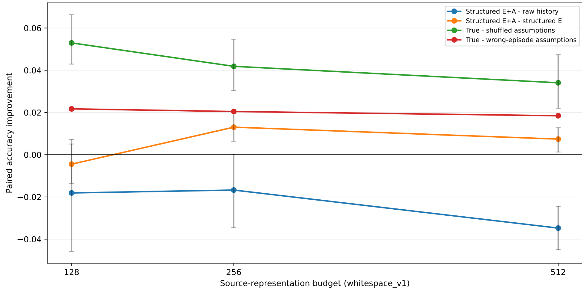
Structured-state lifts over matched controls (horizon 1)
