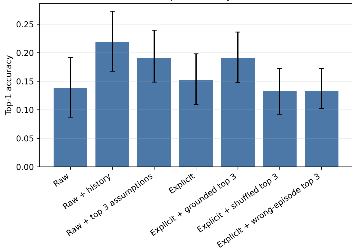
Pairwise representation comparison - complete cases (n=210)
