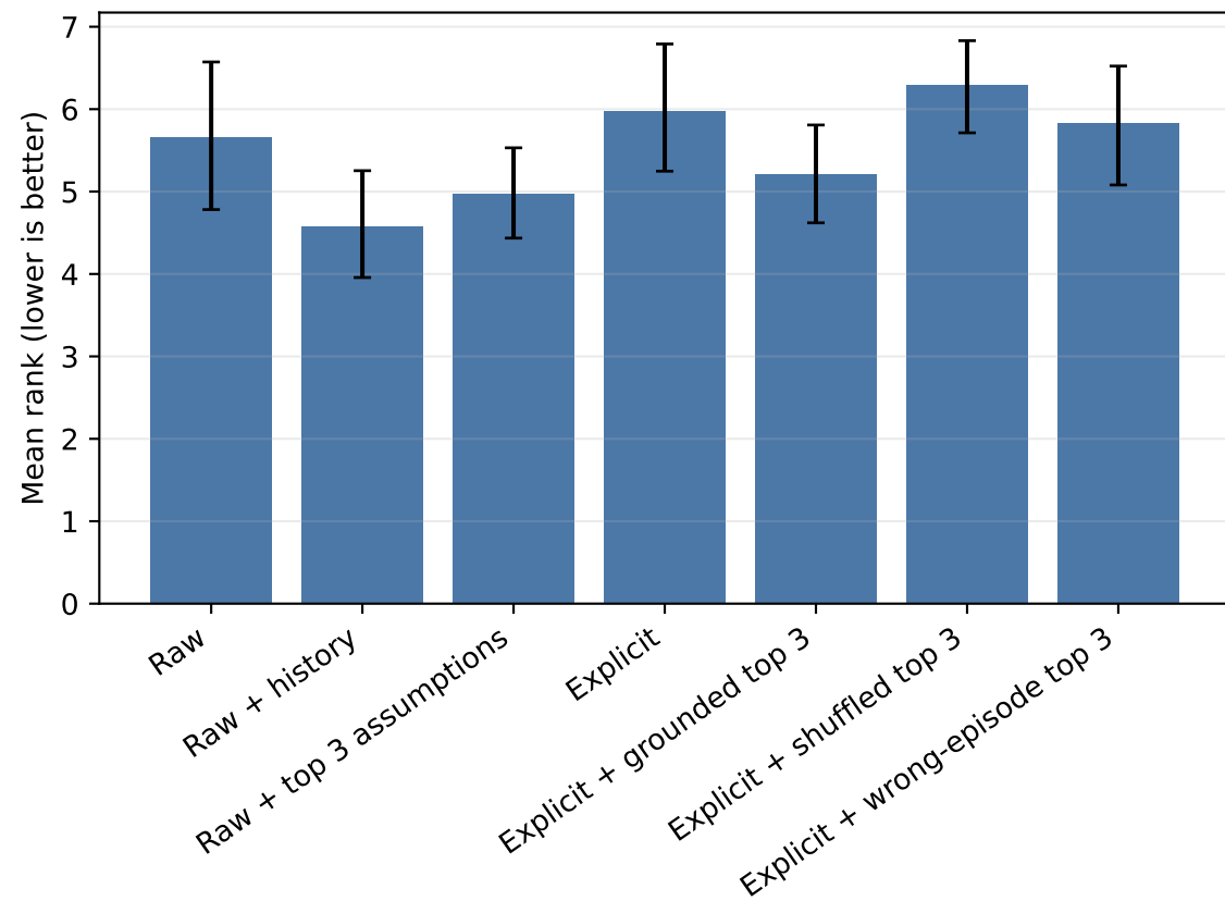
Pairwise representation comparison - complete cases (n=210)
