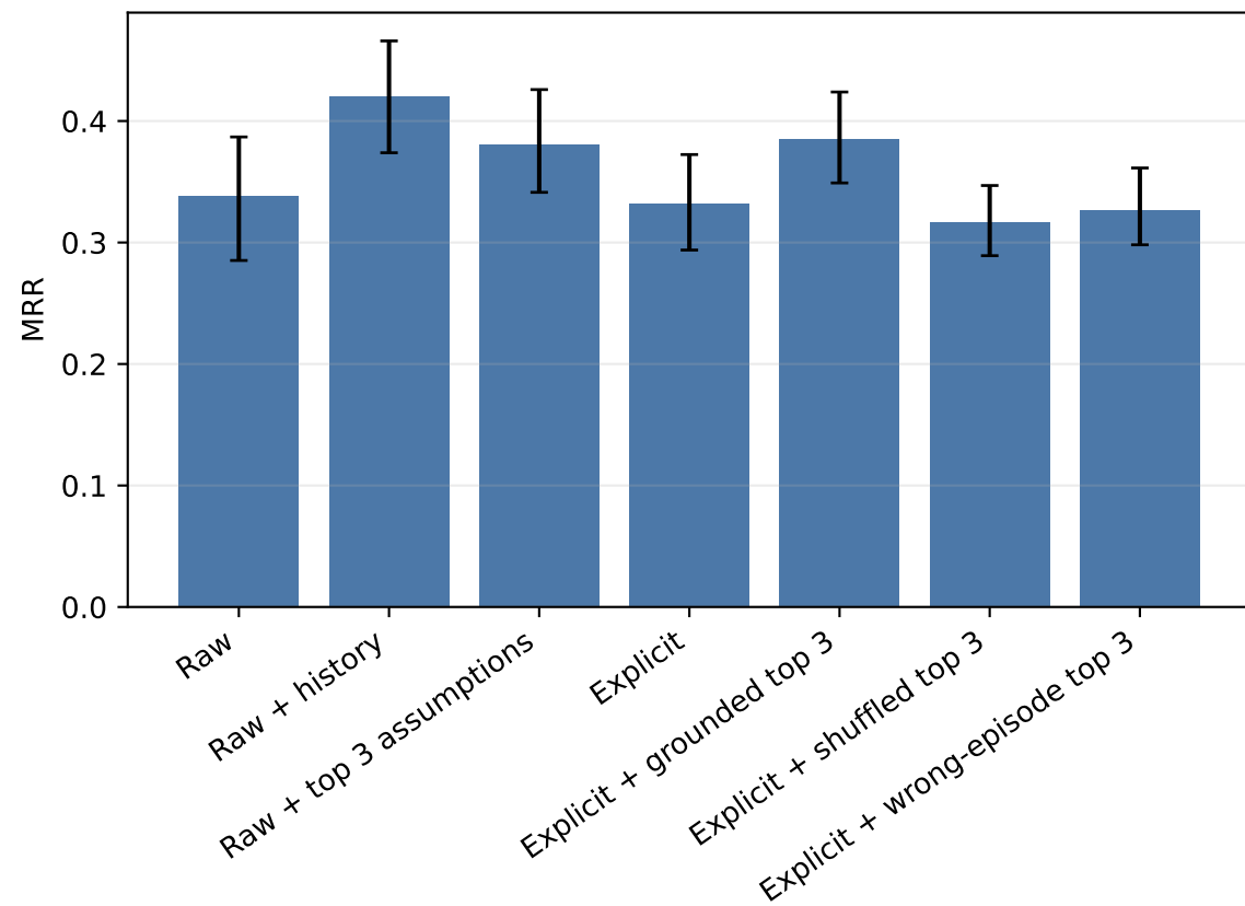
MRR
