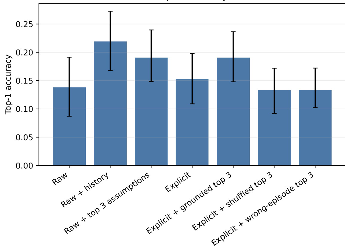
Top-1 accuracy
