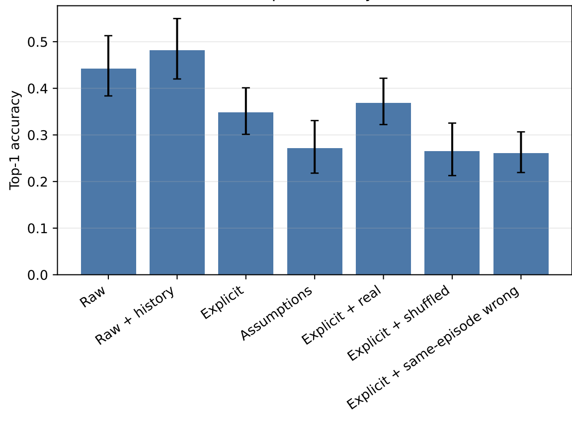
Top-1 accuracy
