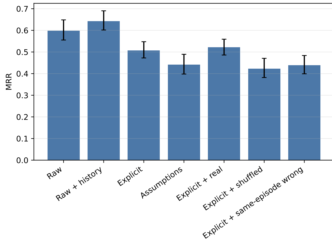
MRR
