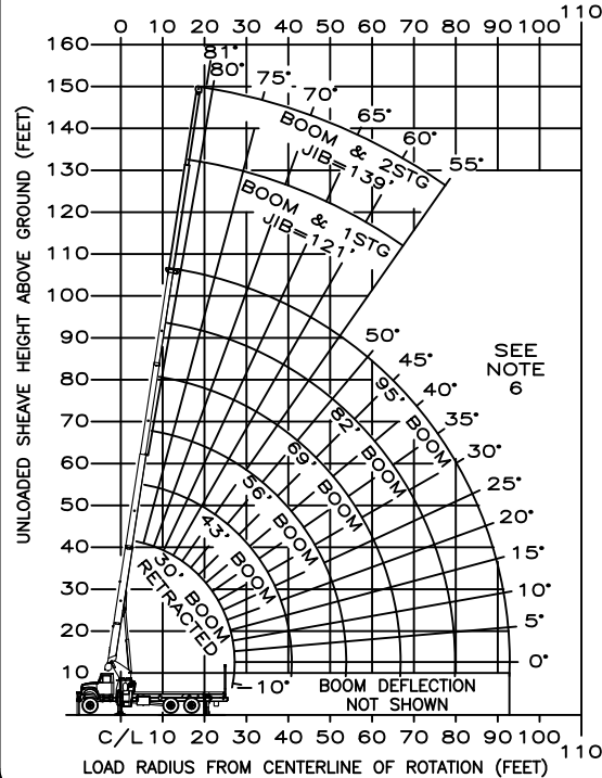
RANGE DIAGRAM - FULL SPAN OUTRIGGERS
