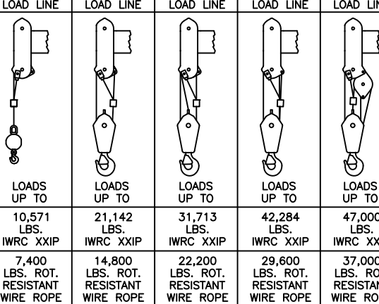
1 PART LOAD LINE 2 PART LOAD LINE 3 PART LOAD LINE 4 PART LOAD LINE 5 PART LOAD LINE
