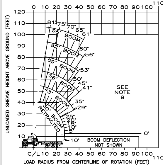
RANGE DIAGRAM - SHORT SPAN OUTRIGGERS
