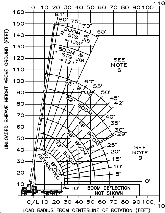
RANGE DIAGRAM - MID SPAN OUTRIGGERS
