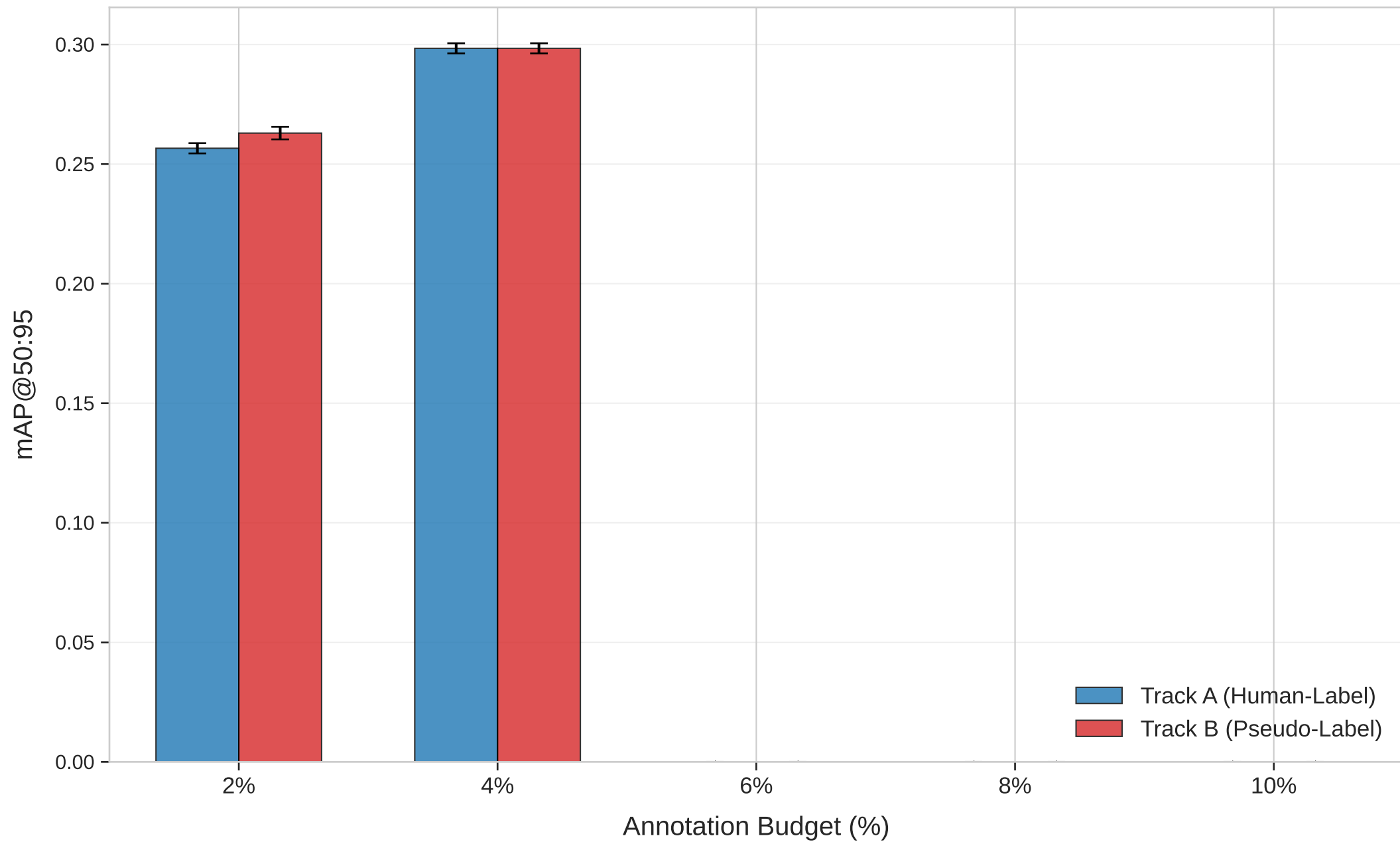
Track A vs Track B: mAP50@95 by Budget
