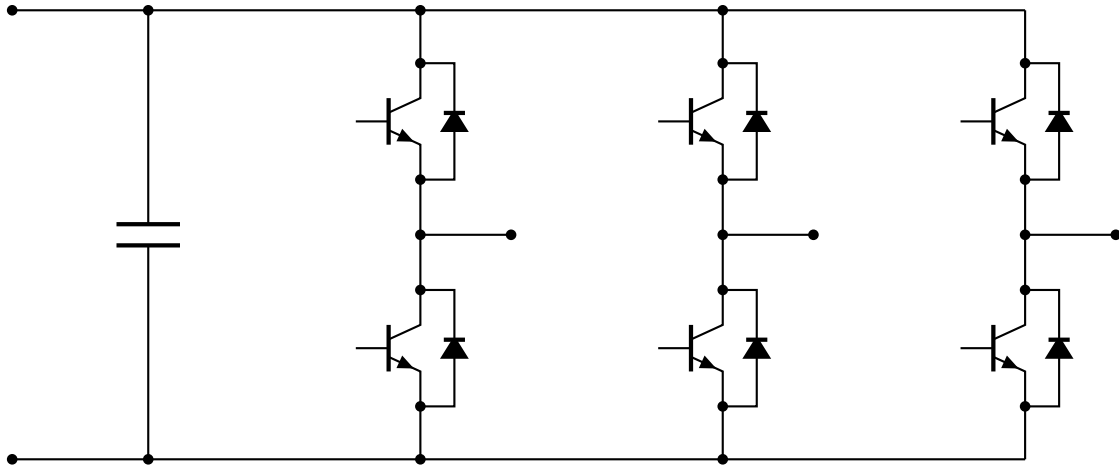
Figure 1: Three-Phase Voltage Source Inverter Bridge
