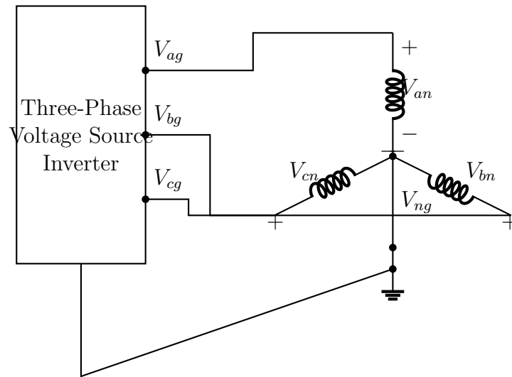
Figure 2: Three-Phase Voltage Source Inverter Feeding a Y-Connected Load
