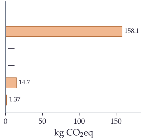
Data preparation
