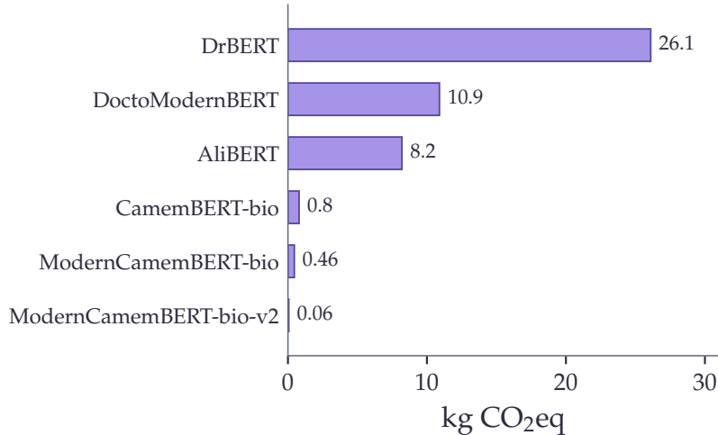
Model training
