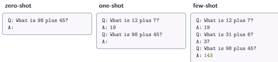
Figure 5.7: The same question put to GPT-3 in three ways. With no example (zero-shot) the model sees only the question; with one or a few solved examples in the prompt (one- and few-shot) it picks up the pattern and answers (in green). No weights are updated; the examples are just text. The format and the final example are from Brown et al. (2020) .
