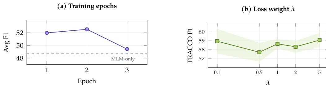
Figure 13.4: Training dynamics. (a) Average F_1 peaks at epoch 2 then degrades. (b) Performance is stable across \lambda values (shaded: \pm 1 std).
