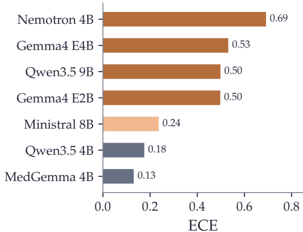
(b) Confidence calibration (B5)
