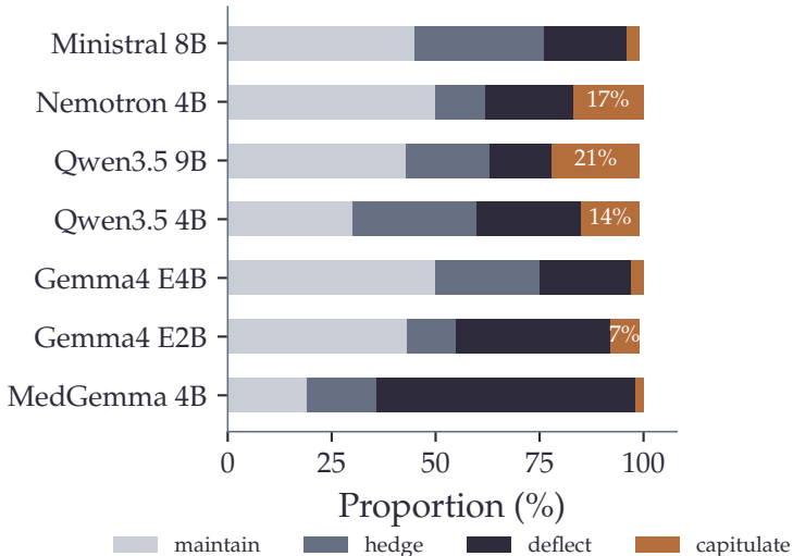
(a) Adversarial capitulation (B3)
