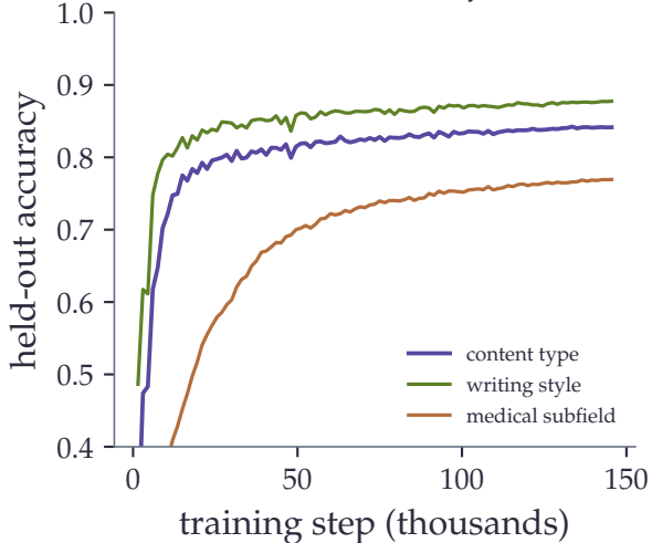
Held-out accuracy
