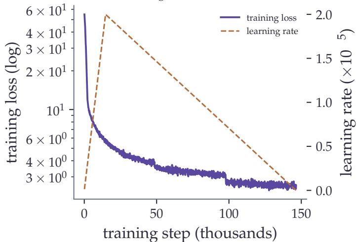
Training loss and schedule
