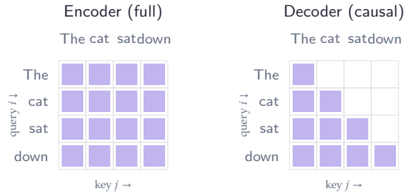
Figure 5.4: Attention masks as matrices. Row i is a query token and column j a key token; a filled cell means token i may attend to token j . The encoder allows every pair, so the matrix is full; the decoder allows only j \leq i , the lower triangle, so each token sees itself and the tokens before it but none of those that follow.
