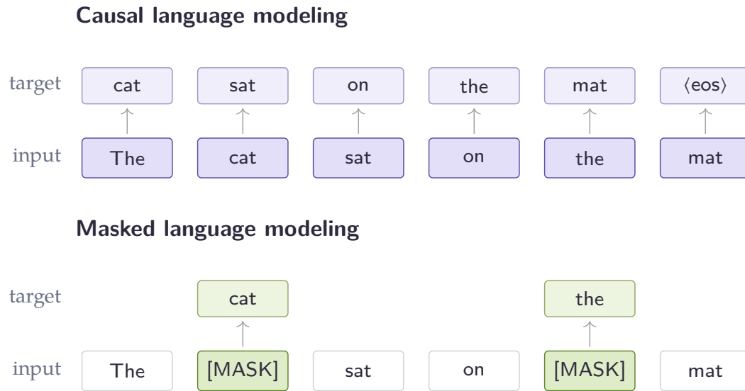
Figure 5.5: The same sentence under the two objectives. The bottom row is the input and the boxes above are the targets the model must predict, one arrow per predicted position. Causal language modeling predicts the next token at every position, so every token gives a training signal (dense). Masked language modeling hides about 15% of the tokens, here two, and predicts only those from the context on both sides, so most positions give no signal (sparse). This gap in how much signal each token carries is what the encoder pretraining of Chapter 12 exploits.
