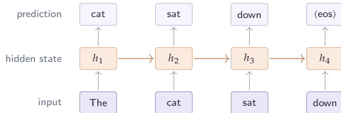
Figure 5.4: A recurrent language model, drawn one step per token. At each position the network combines the current input with the hidden state carried over from the previous step (the horizontal arrows) and predicts the next token, so the running state lets a prediction depend on the whole past rather than a fixed window.
