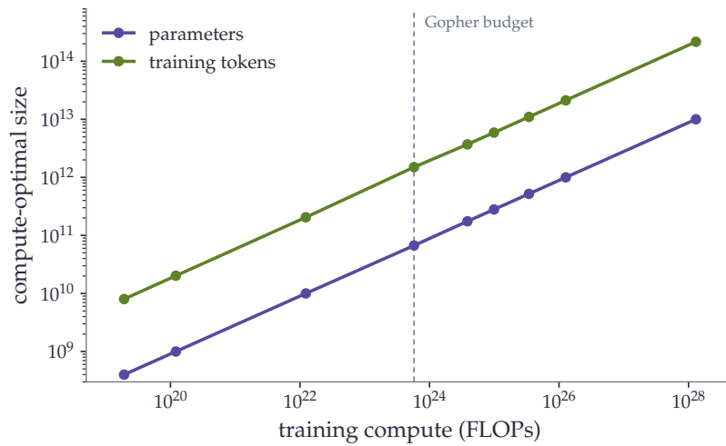
Figure 5.9: The compute-optimal model size and the compute-optimal number of training tokens rise together with the training budget, as the parallel lines show. Points are verbatim from Table 3 of Hoffmann et al. (2022) ; the paper’s loss curves are not reproduced here.
