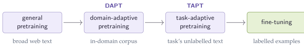
Figure 5.11: Continued pretraining inserts one or two self-supervised phases between general pretraining and fine-tuning: domain-adaptive pretraining on a large in-domain corpus, then task-adaptive pretraining on the task’s own unlabelled text ( Gururangan et al., 2020 ).
