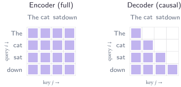
Figure 4.6: Attention masks as matrices. Row i is a query token and column j a key token; a filled cell means token i may attend to token j . The encoder allows every pair, so the matrix is full; the decoder allows only j \leq i , the lower triangle, so each token sees itself and the tokens before it but none of those that follow.
