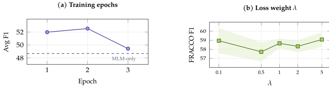
Figure 12.4: Training dynamics. (a) Average F_1 peaks at epoch 2 then degrades. (b) Performance is stable across \lambda values (shaded: \pm 1 std).
