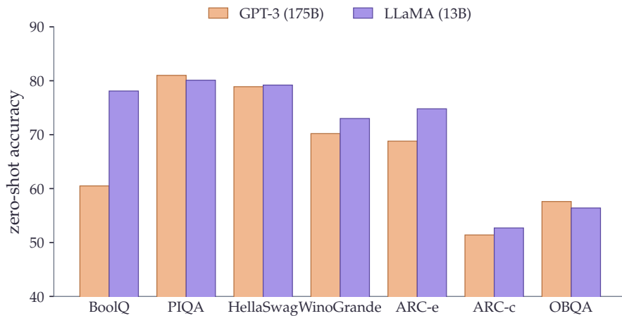
Figure 4.10: A 13-billion-parameter model trained on more tokens matches or beats GPT-3, which is more than ten times larger, on most of these zero-shot reasoning tasks. Numbers are from Table 3 of Touvron et al. (2023) .
